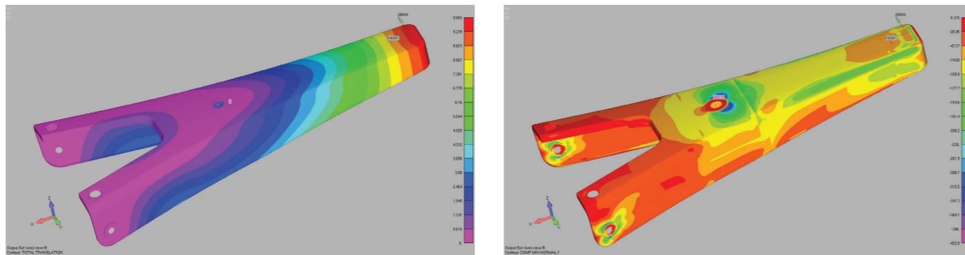
Finite Element Analysis of the bowsprit to simulate stress under different load conditions (Source: Asta)
